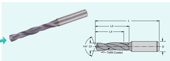
HQS Drill Point
