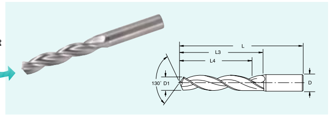
TF Drill Point
