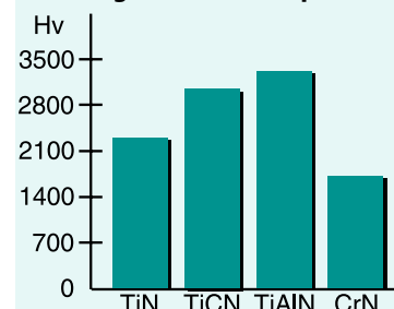
Coating Hardness Comparison
